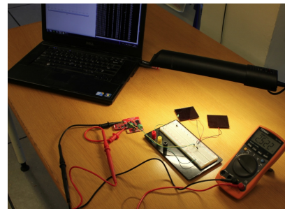
Figure 1: Ex. of Nodes in our EH-WSN Test-Bed
